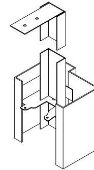
Plaster Partition Anchor (Ceiling Strut Optional)
