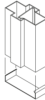
Typical Mullion Sections with Base Anchor
